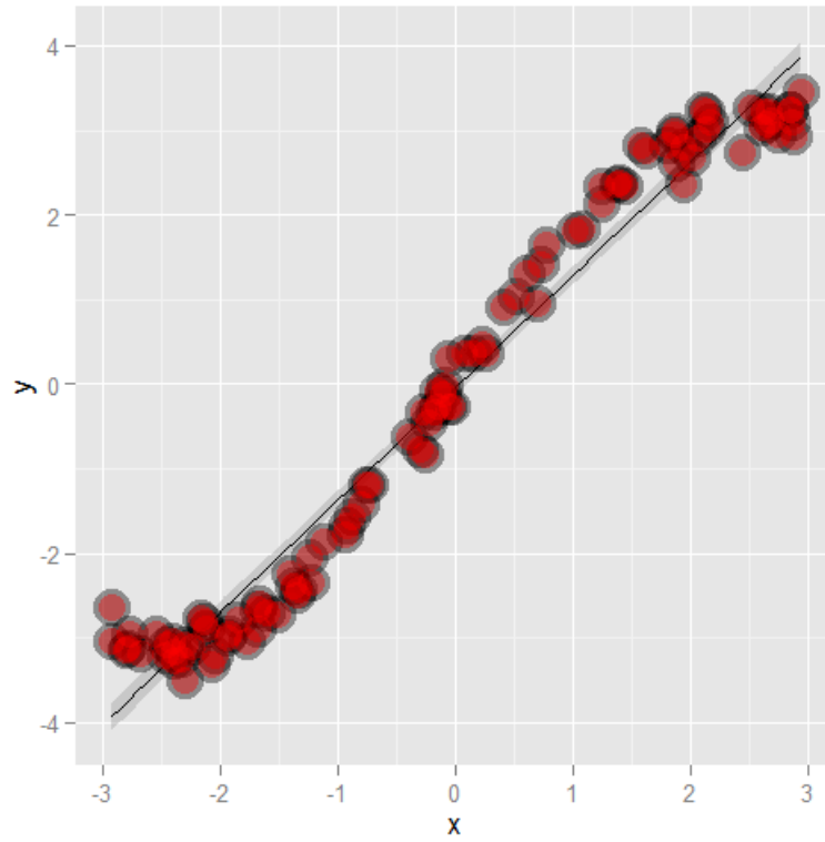
Plot of simulated non-linear data.
